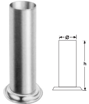
Metal without lid \varnothing 100 \times 175 mm (1pc)
